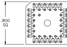
44 Pin Adapter Closed Frame P/N ADP-000011 (GOLD PINS) P/N ADP-000011T (TIN PINS)
