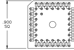
52 Pin Adapter Closed Frame P/N ADP-000012 (GOLD PINS) P/N ADP-000012T (TIN PINS)
