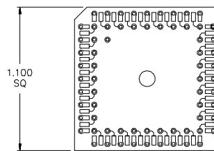
68 Pin Adapter Closed Frame P/N ADP-000013 (GOLD PINS) P/N ADP-000013T (TIN PINS)
