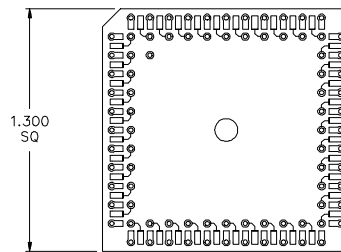
84 Pin Adapter Open Frame P/N ADP-000004 (GOLD PINS) P/N ADP-000004T (TIN PINS)
