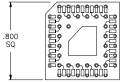
44 Pin Adapter Open Frame P/N ADP-000003 (GOLD PINS) P/N ADP-000003T (TIN PINS)
