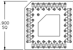
52 Pin Adapter Open Frame P/N ADP-000005 (GOLD PINS) P/N ADP-000005T (TIN PINS)
