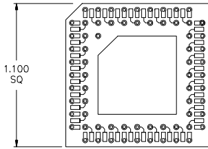
68 Pin Adapter Open Frame P/N ADP-000006 (GOLD PINS) P/N ADP-000006T (TIN PINS)
