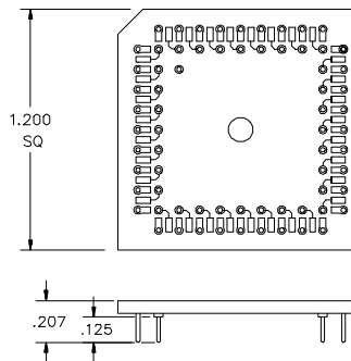
68 Pin Adapter Closed Frame P/N ADP-000029 (GOLD PINS) P/N ADP-000029T (TIN PINS)
