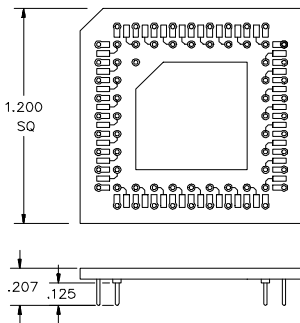
68 Pin Adapter Open Frame P/N ADP-000021 (GOLD PINS) P/N ADP-000021T (TIN PINS)
