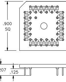
44 Pin Adapter Closed Frame P/N ADP-000027 (GOLD PINS) P/N ADP-000027T (TIN PINS)
