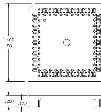
84 Pin Adapter Open Frame P/N ADP-000022 (GOLD PINS) P/N ADP-000022T (TIN PINS)
