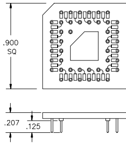
44 Pin Adapter Open Frame P/N ADP-000019 (GOLD PINS) P/N ADP-000019T (TIN PINS)
