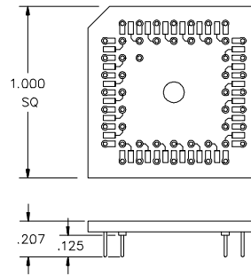
52 Pin Adapter Closed Frame P/N ADP-000028 (GOLD PINS) P/N ADP-000028T (TIN PINS)
