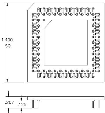
84 Pin Adapter Open Frame P/N ADP-000022 (GOLD PINS) P/N ADP-000022T (TIN PINS)
