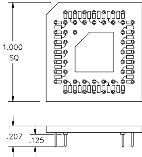
52 Pin Adapter Open Frame P/N ADP-000020 (GOLD PINS) P/N ADP-000020T (TIN PINS)
