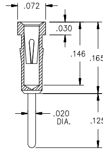
PIN STYLE 0011J FOR PGA'S WITH PIN COUNTS UPTO 145
