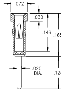
PIN STYLE 0011K FOR PGA'S WITH PIN COUNTS OVER 145
