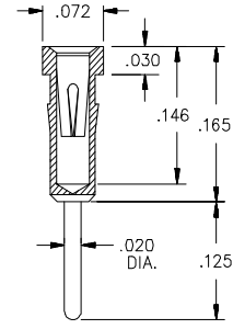
PIN STYLE 0011L FOR PGA'S WITH PIN COUNTS OVER 400
